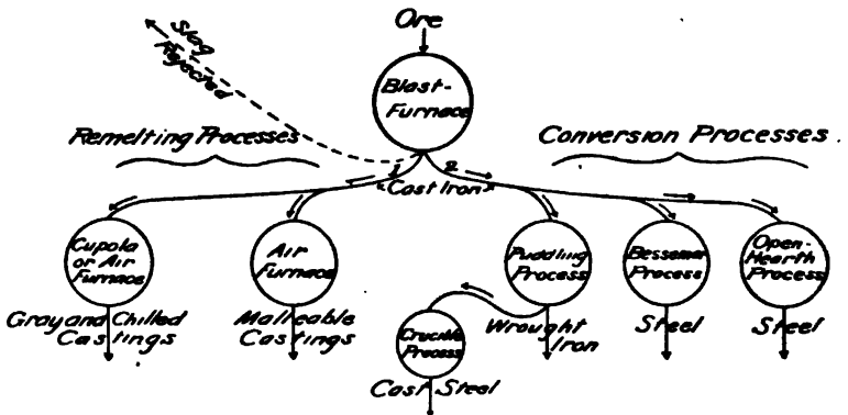
Fig. 87. The General Scheme of Iron Manufacture.
